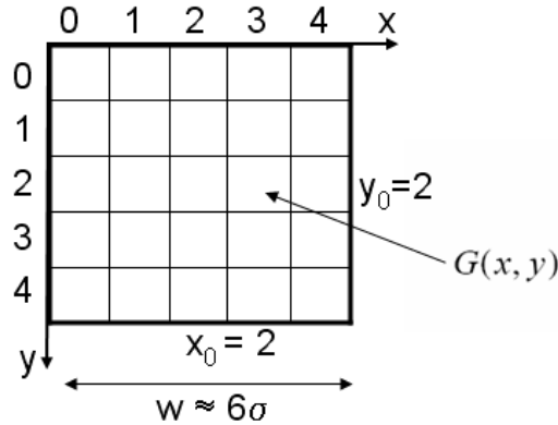
Fig. 10.4 Design example of a Gaussian kernel/filter having a 5x5 size.
