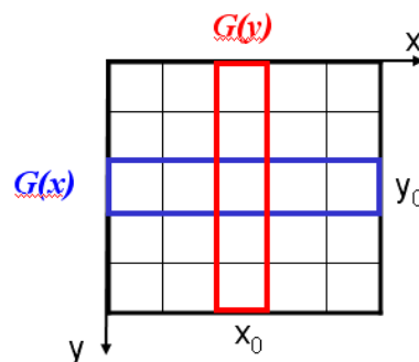
Fig. 10.5 The two vectors G(x) and G(y) into which a 2D Gaussian kernel may be separated
